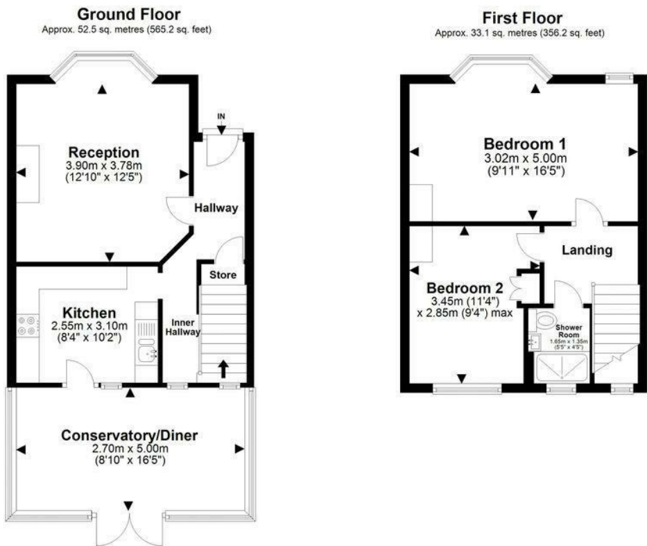
Total area: approx. 85.6 sq. metres (921.4 sq. feet) All images used are for illustrative purposes only. Floor plans are intended to give a general indication of the proposed layout only. All images and dimensions are not intended to form part any contract or warranty. Plan produced using PlanUp.
